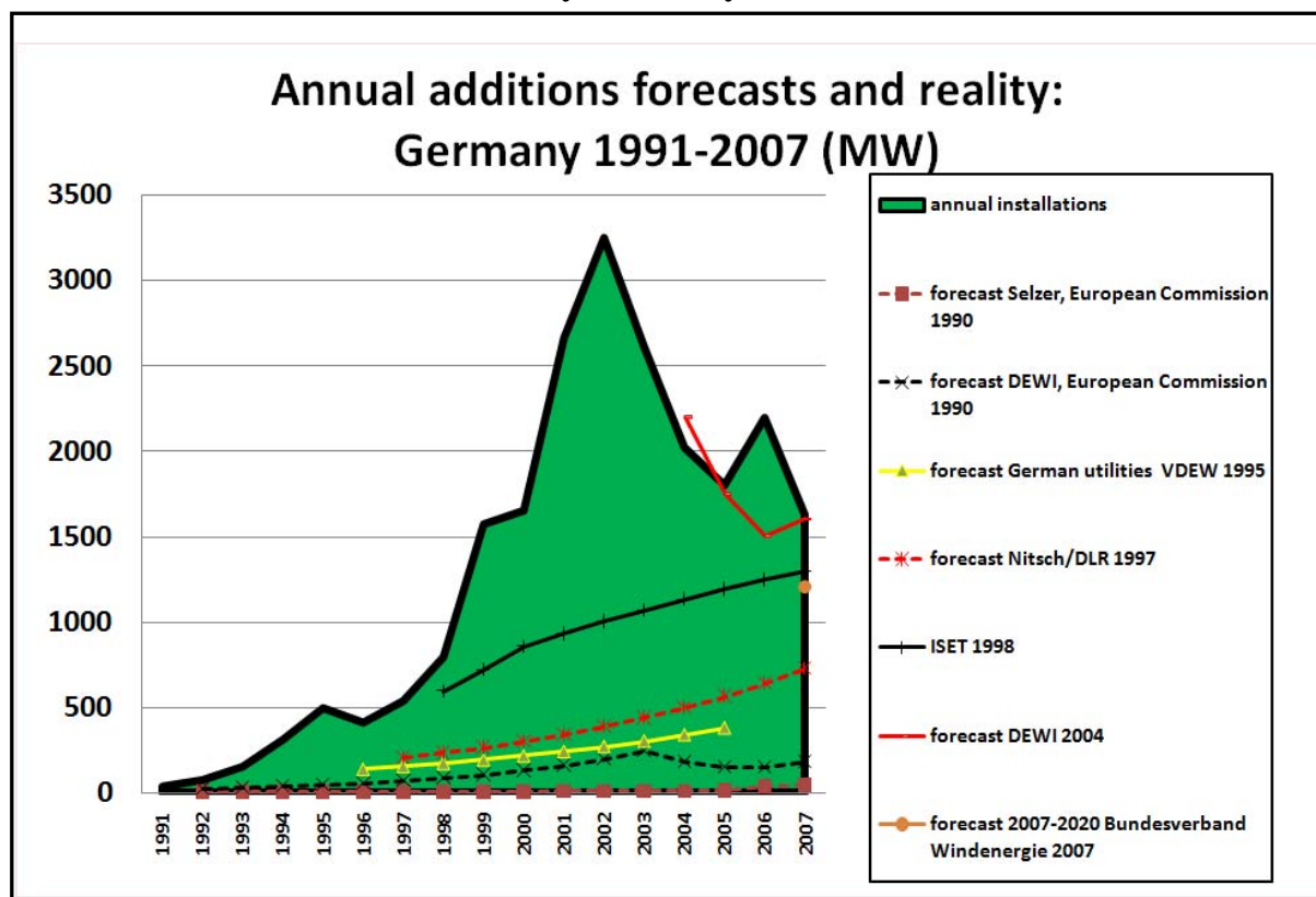
Figure 63 Annual additions forecasts and reality: Germany 1991-2007
