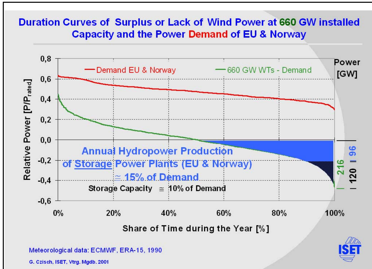
Figure 158 excess power and storage needs for Europe calculated by Gregor Czisch source: Czisch / ISET
