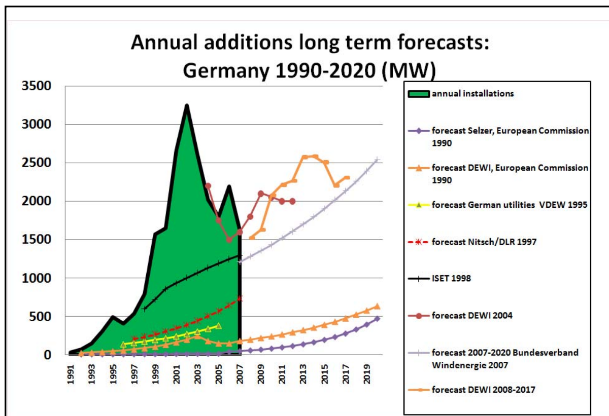
Figure 66 Long-term forecasts for annual additions: Germany
